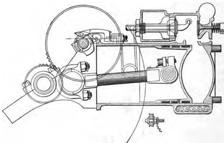
FIG. 227—Sectional View through One Cylinder of the Durvea Three-Cylinder Engine, showing working parts. The exhaust cam operated by a two-to-one gear imparts a double motion to the valve pushrod; a lift for opening the valve, and a double twist for making and breaking the connections of the electrical spark. The valve and sparking chamber is projected so as to show the position of contained mechanism on a plane different from that of the cylinder section. Details of the insulated sparking anvil are shown below the cylinder. It is an iron contact point, having a mica washer on the inside and the outside of the cylinder walls, and a mica bushing between, so as to perfectly insulate it from the metal of the engine. A very short water jacket and the concave cylinder and piston heads are also exhibited in this figure.
